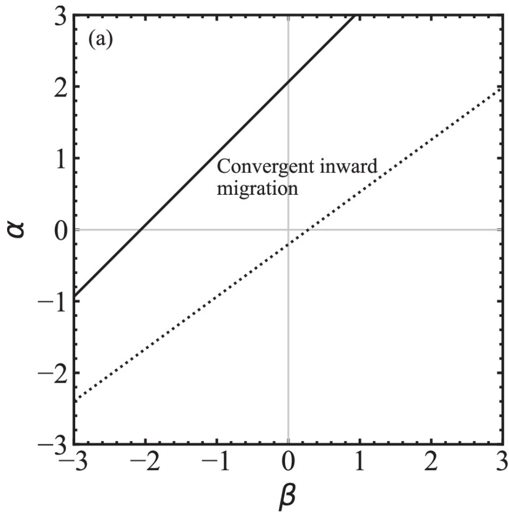
Figure 2. from Ka Ho Wong and Man Hoi Lee 2024 Astron. J. 167 doi:10.3847/1538-3881/ad1f60 https://dx.doi.org/10.3847/1538-3881/ad1f60 © 2024. The Author(s). Published by the American Astronomical Society.
