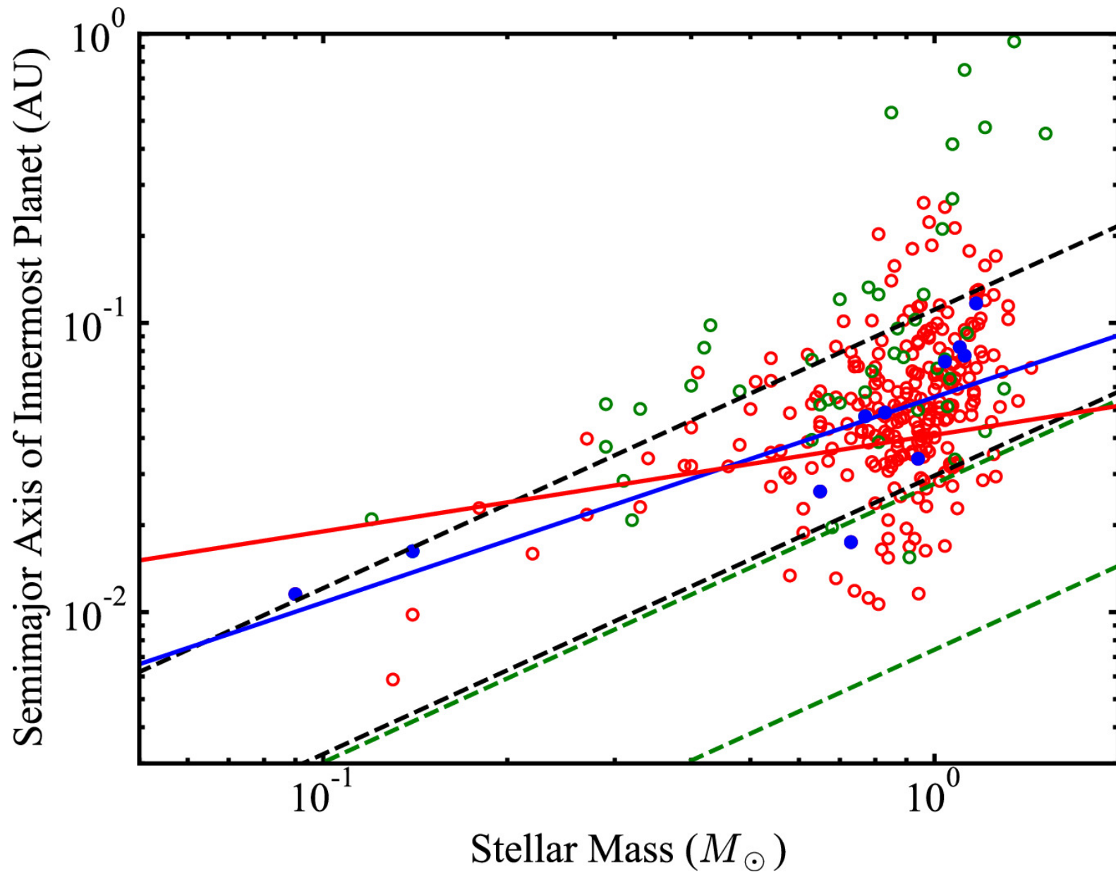
Figure 10. from Ka Ho Wong and Man Hoi Lee 2024 Astron. J. 167 doi:10.3847/1538-3881/ad1f60 https://dx.doi.org/10.3847/1538-3881/ad1f60 © 2024. The Author(s). Published by the American Astronomical Society.
