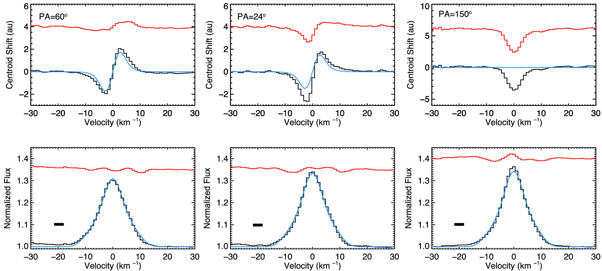
Figure 6. from Stanley K. Jensen et al 2024 Astron. J. 167 doi:10.3847/1538-3881/ad1b5d https://dx.doi.org/10.3847/1538-3881/ad1b5d © 2024. The Author(s). Published by the American Astronomical Society.
