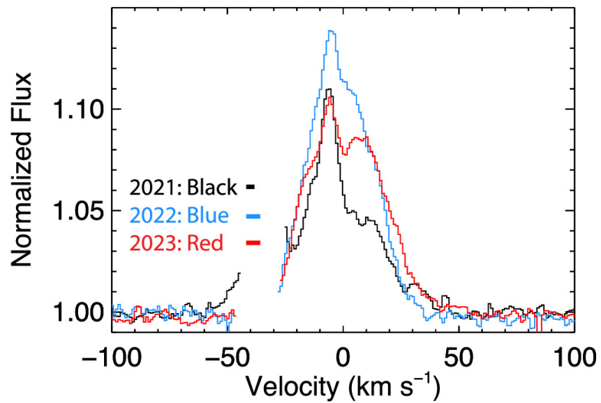
Figure 4. from Stanley K. Jensen et al 2024 Astron. J. 167 doi:10.3847/1538-3881/ad1b5d https://dx.doi.org/10.3847/1538-3881/ad1b5d © 2024. The Author(s). Published by the American Astronomical Society.
