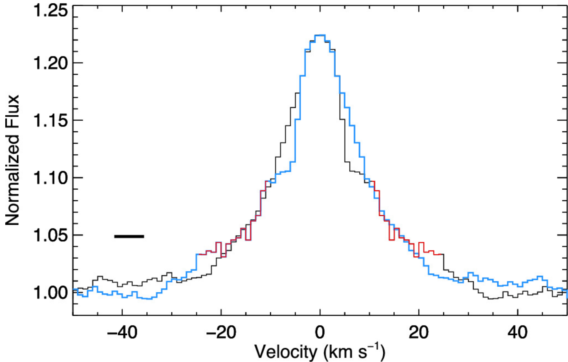
Figure 3. from Stanley K. Jensen et al 2024 Astron. J. 167 doi:10.3847/1538-3881/ad1b5d https://dx.doi.org/10.3847/1538-3881/ad1b5d © 2024. The Author(s). Published by the American Astronomical Society.
