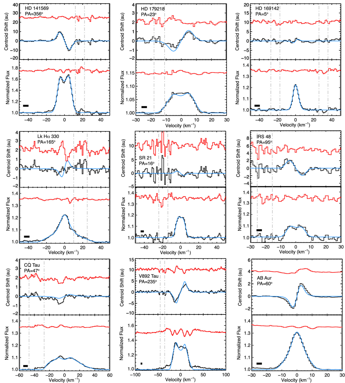
Figure 1. from Stanley K. Jensen et al 2024 Astron. J. 167 doi:10.3847/1538-3881/ad1b5d https://dx.doi.org/10.3847/1538-3881/ad1b5d © 2024. The Author(s). Published by the American Astronomical Society.
