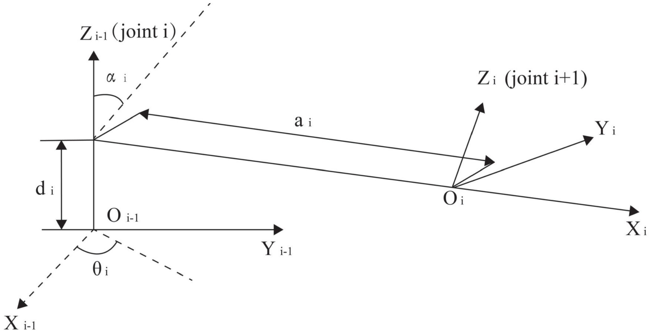
Figure 4. from Feifan Zhang et al 2024 Astron. J. 167 doi:10.3847/1538-3881/ad1b4d https://dx.doi.org/10.3847/1538-3881/ad1b4d © 2024. The Author(s). Published by the American Astronomical Society.
