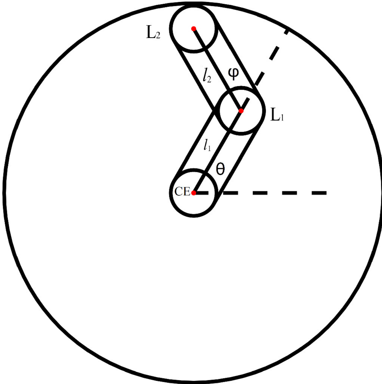
Figure 3. from Feifan Zhang et al 2024 Astron. J. 167 doi:10.3847/1538-3881/ad1b4d https://dx.doi.org/10.3847/1538-3881/ad1b4d © 2024. The Author(s). Published by the American Astronomical Society.
