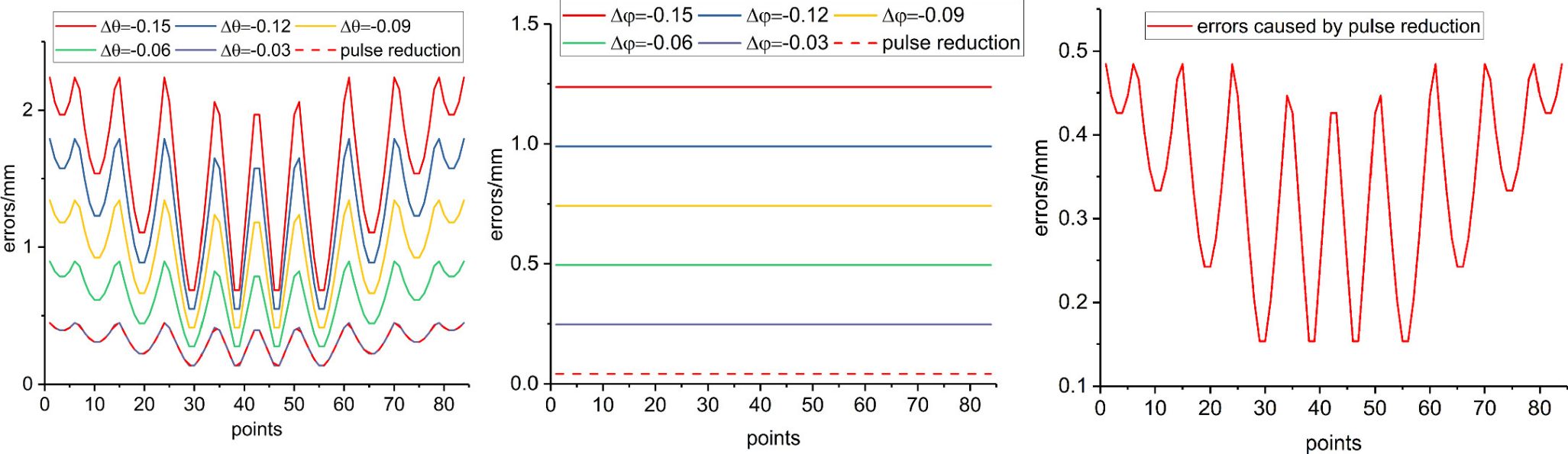
Figure 10. from Feifan Zhang et al 2024 Astron. J. 167 doi:10.3847/1538-3881/ad1b4d https://dx.doi.org/10.3847/1538-3881/ad1b4d © 2024. The Author(s). Published by the American Astronomical Society.
