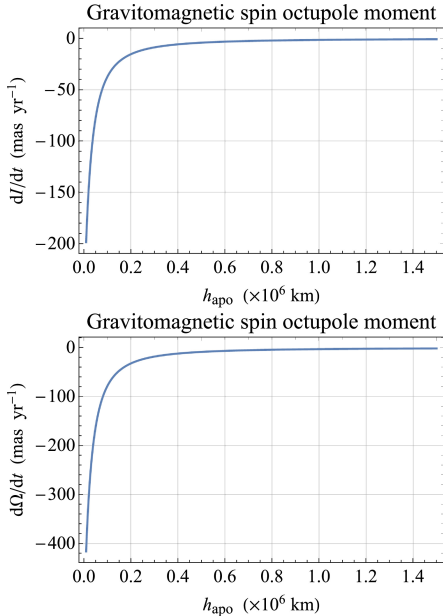
Figure 6. from Lorenzo Iorio 2024 Astron. J. 167 doi:10.3847/1538-3881/ad1833 https://dx.doi.org/10.3847/1538-3881/ad1833 © 2024. The Author(s). Published by the American Astronomical Society.
