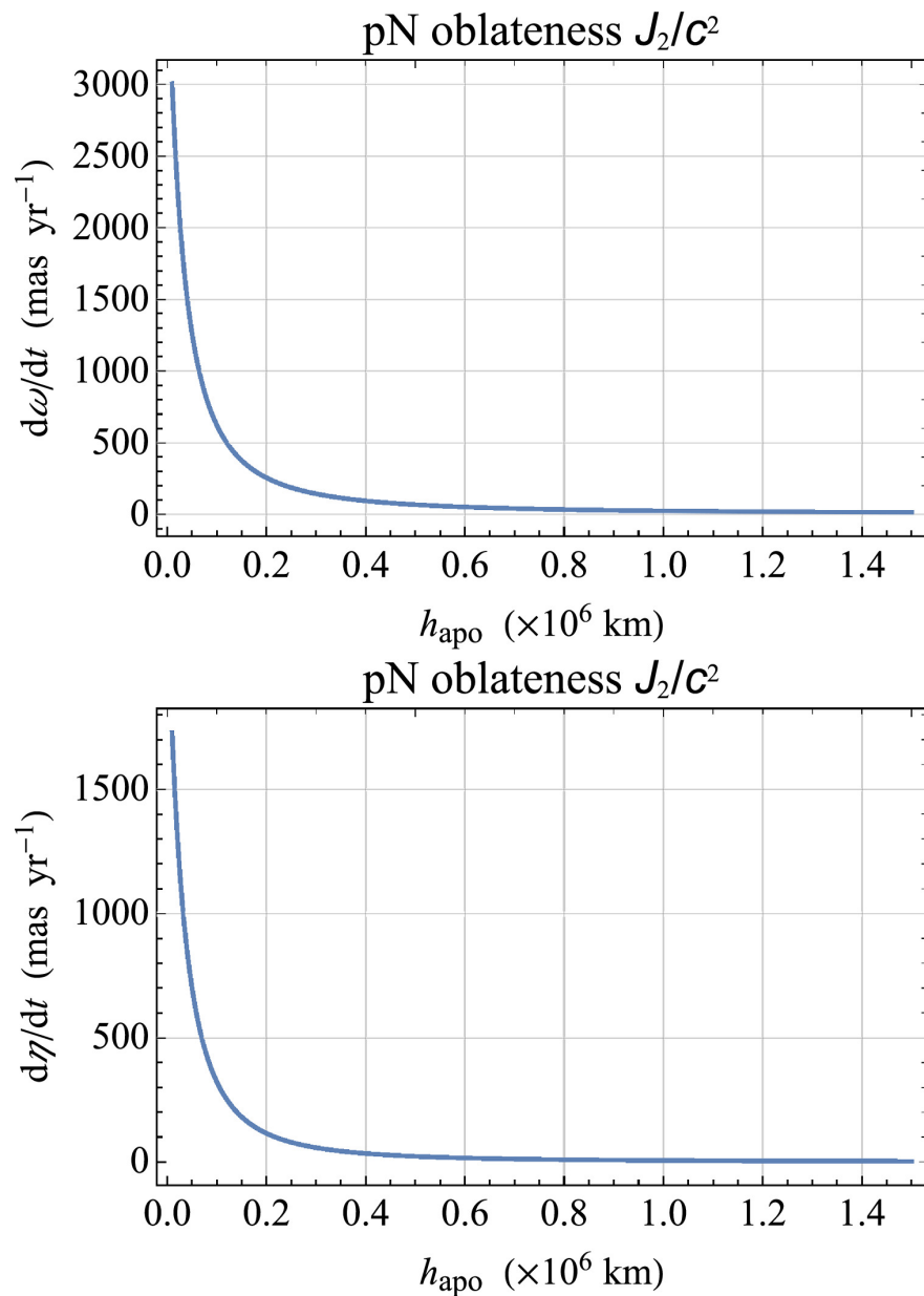
Figure 5. from Lorenzo Iorio 2024 Astron. J. 167 doi:10.3847/1538-3881/ad1833 https://dx.doi.org/10.3847/1538-3881/ad1833 © 2024. The Author(s). Published by the American Astronomical Society.
