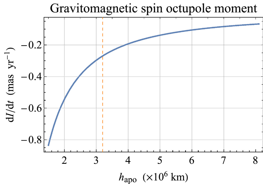
Figure 3. from Lorenzo Iorio 2024 Astron. J. 167 doi:10.3847/1538-3881/ad1833 https://dx.doi.org/10.3847/1538-3881/ad1833 © 2024. The Author(s). Published by the American Astronomical Society.
