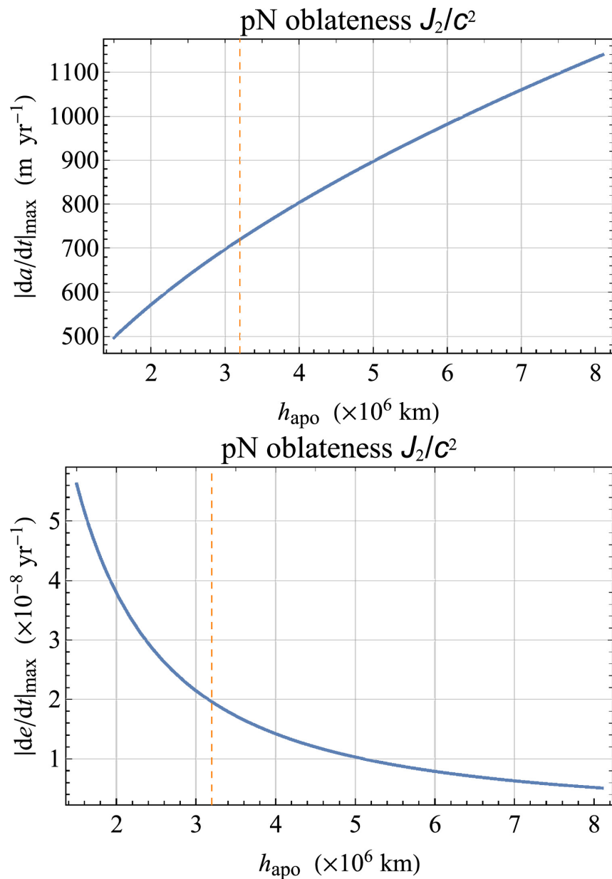
Figure 1. from Lorenzo Iorio 2024 Astron. J. 167 doi:10.3847/1538-3881/ad1833 https://dx.doi.org/10.3847/1538-3881/ad1833 © 2024. The Author(s). Published by the American Astronomical Society.
