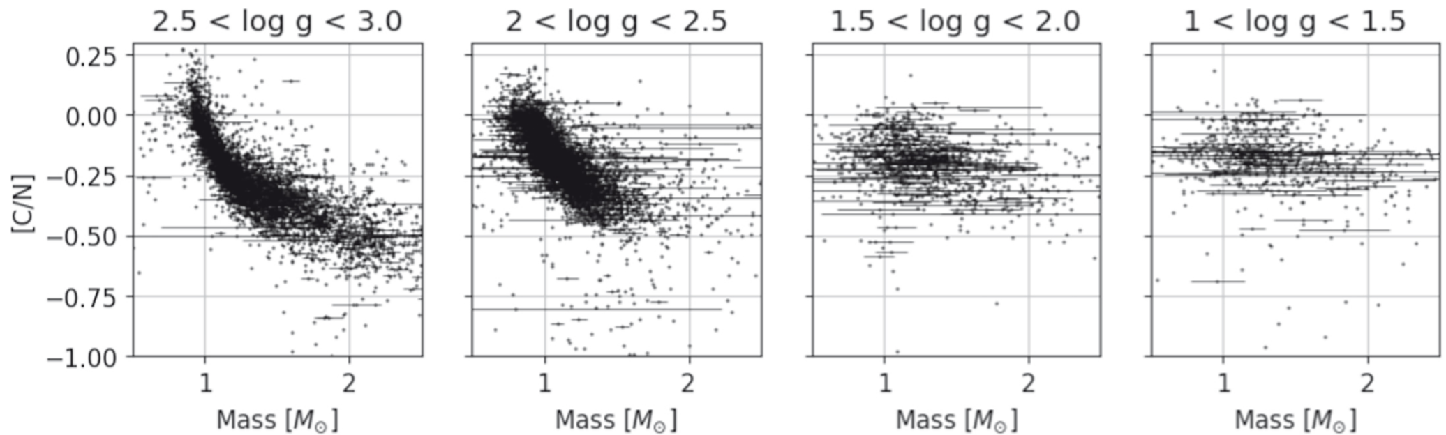
Figure 7. from Alexander Stone-Martinez et al 2024 Astron. J. 167 doi:10.3847/1538-3881/ad12a6 https://dx.doi.org/10.3847/1538-3881/ad12a6 © 2024. The Author(s). Published by the American Astronomical Society.
