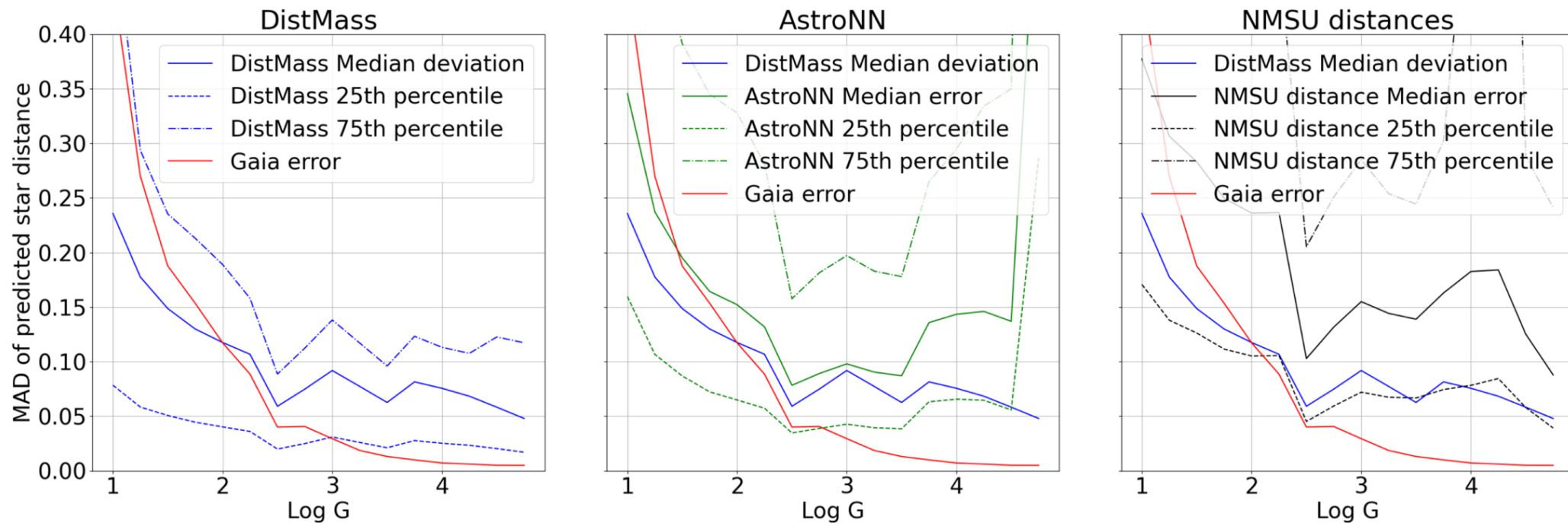
Figure 4. from Alexander Stone-Martinez et al 2024 Astron. J. 167 doi:10.3847/1538-3881/ad12a6 https://dx.doi.org/10.3847/1538-3881/ad12a6 © 2024. The Author(s). Published by the American Astronomical Society.
