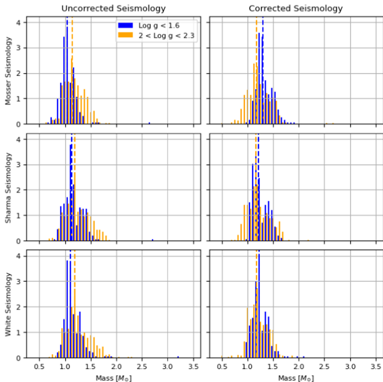
Figure 14. from Alexander Stone-Martinez et al 2024 Astron. J. 167 doi:10.3847/1538-3881/ad12a6 https://dx.doi.org/10.3847/1538-3881/ad12a6 © 2024. The Author(s). Published by the American Astronomical Society.
