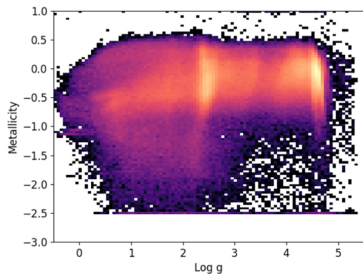
(c) Full data set log g vs metallicity
