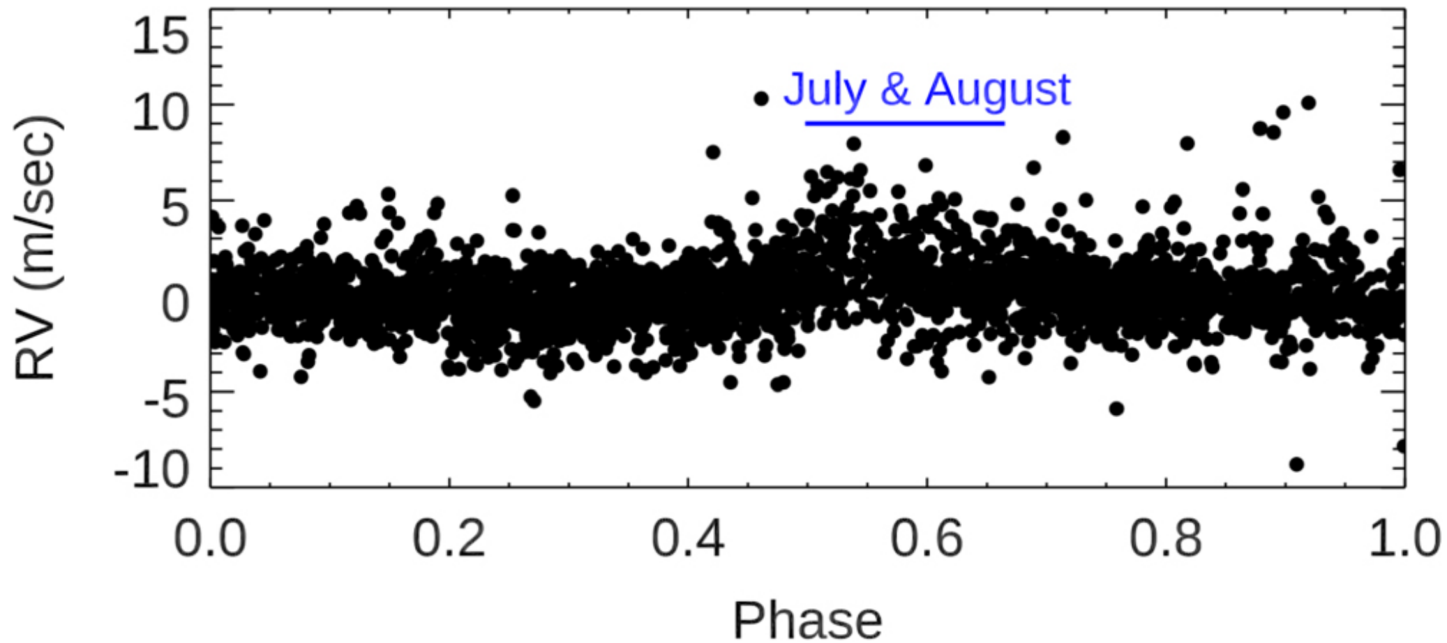
Figure 9. from Drake Deming et al 2024 Astron. J. 167 doi:10.3847/1538-3881/ad109f https://dx.doi.org/10.3847/1538-3881/ad109f © 2023. The Author(s). Published by the American Astronomical Society.
