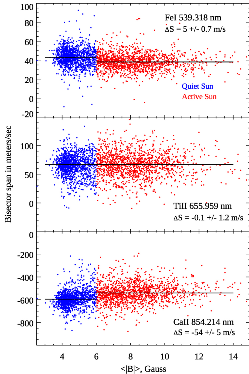
Figure 8. from Drake Deming et al 2024 Astron. J. 167 doi:10.3847/1538-3881/ad109f https://dx.doi.org/10.3847/1538-3881/ad109f © 2023. The Author(s). Published by the American Astronomical Society.
