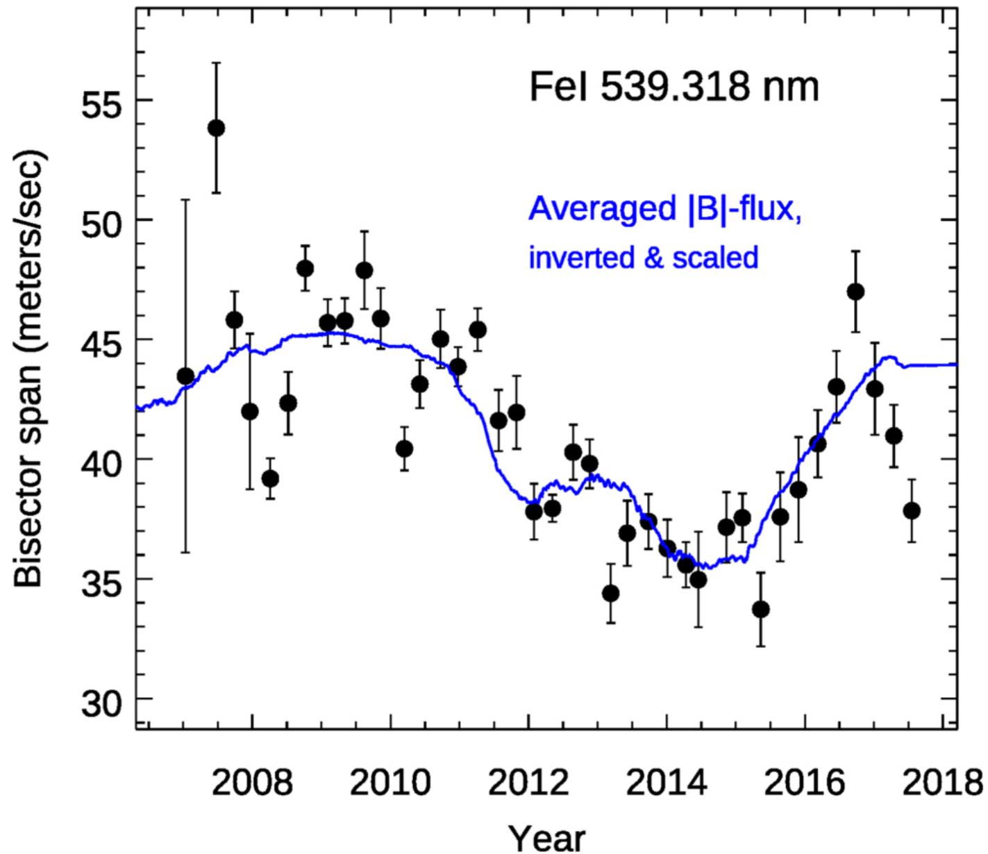
Figure 6. from Drake Deming et al 2024 Astron. J. 167 doi:10.3847/1538-3881/ad109f https://dx.doi.org/10.3847/1538-3881/ad109f © 2023. The Author(s). Published by the American Astronomical Society.
