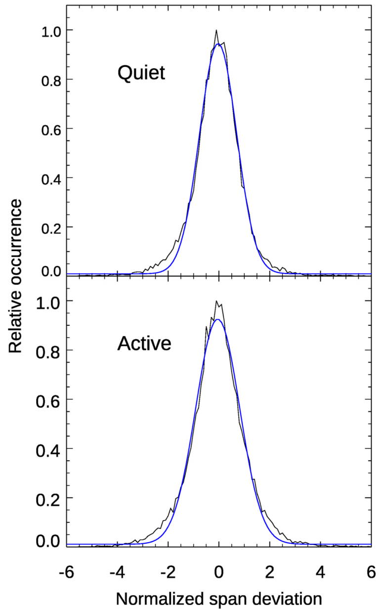
Figure 5. from Drake Deming et al 2024 Astron. J. 167 doi:10.3847/1538-3881/ad109f https://dx.doi.org/10.3847/1538-3881/ad109f © 2023. The Author(s). Published by the American Astronomical Society.
