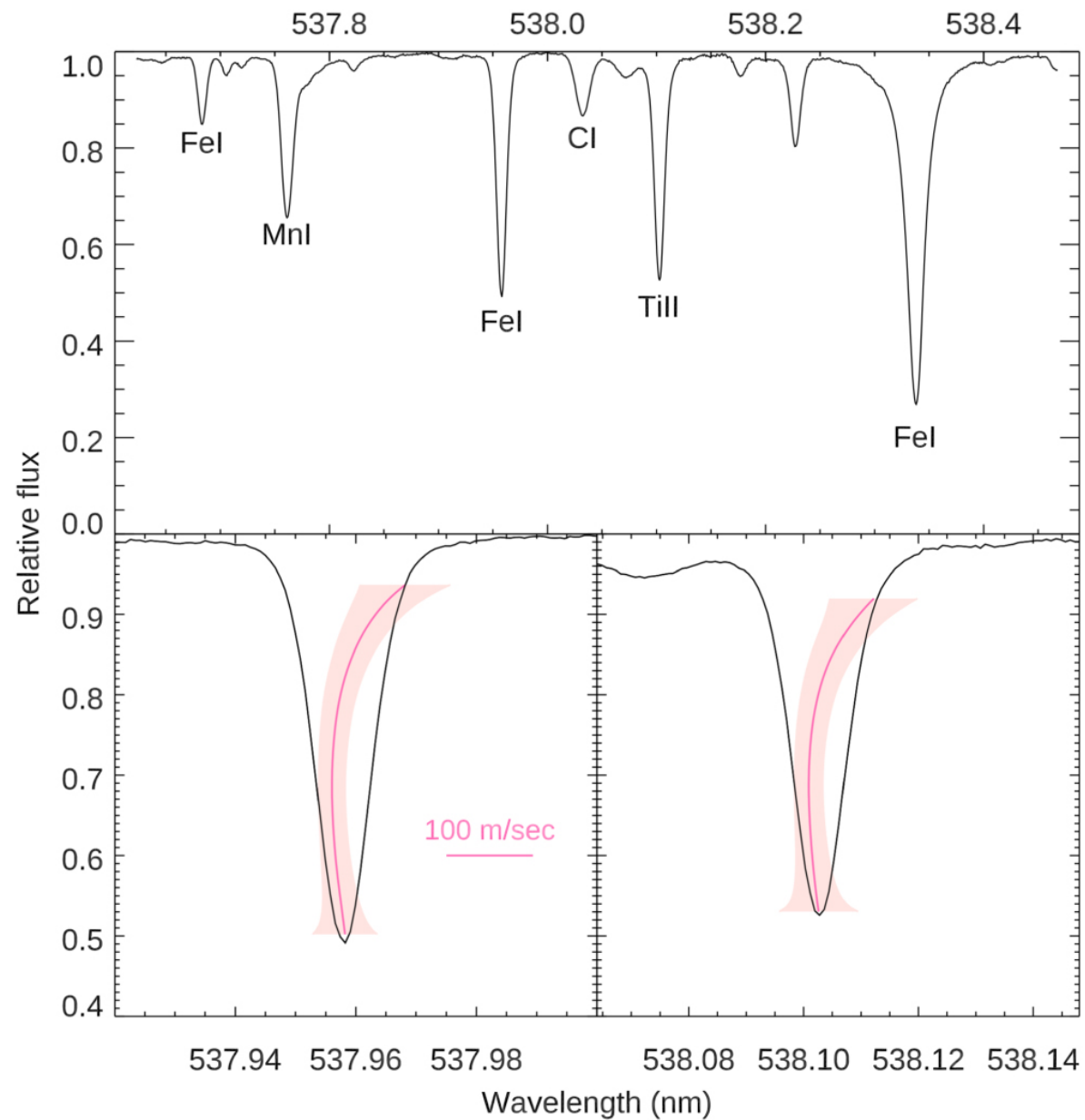
Figure 3. from Drake Deming et al 2024 Astron. J. 167 doi:10.3847/1538-3881/ad109f https://dx.doi.org/10.3847/1538-3881/ad109f © 2023. The Author(s). Published by the American Astronomical Society.
