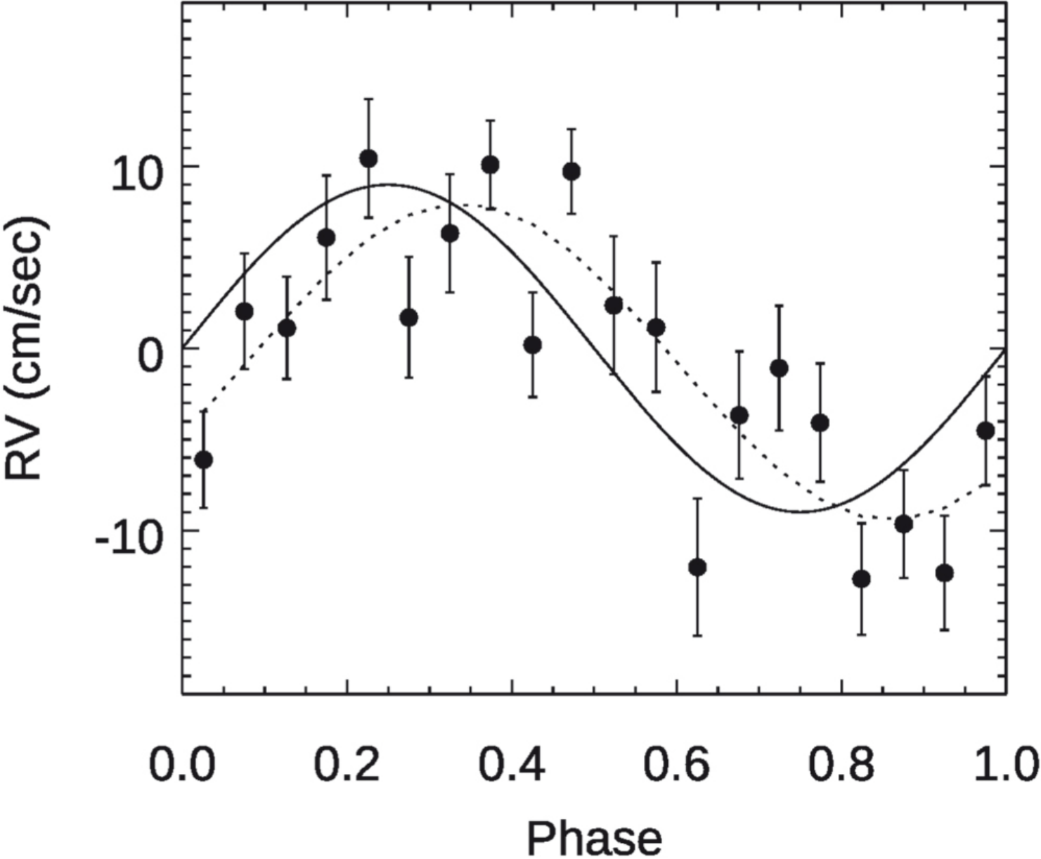
Figure 10. from Drake Deming et al 2024 Astron. J. 167 doi:10.3847/1538-3881/ad109f https://dx.doi.org/10.3847/1538-3881/ad109f © 2023. The Author(s). Published by the American Astronomical Society.
