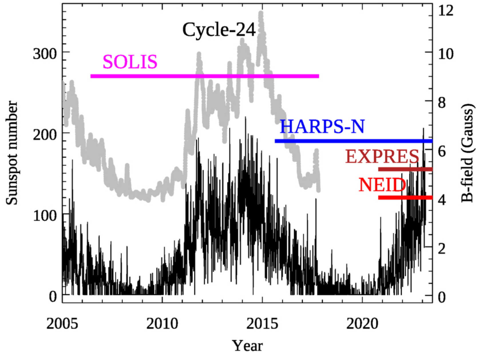
Figure 1. from Drake Deming et al 2024 Astron. J. 167 doi:10.3847/1538-3881/ad109f https://dx.doi.org/10.3847/1538-3881/ad109f © 2023. The Author(s). Published by the American Astronomical Society.
