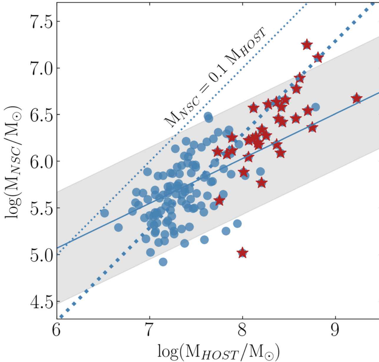
Figure 9. from Mika Lambert et al 2024 Astron. J. 167 doi:10.3847/1538-3881/ad0f25 https://dx.doi.org/10.3847/1538-3881/ad0f25 © 2024. The Author(s). Published by the American Astronomical Society.
