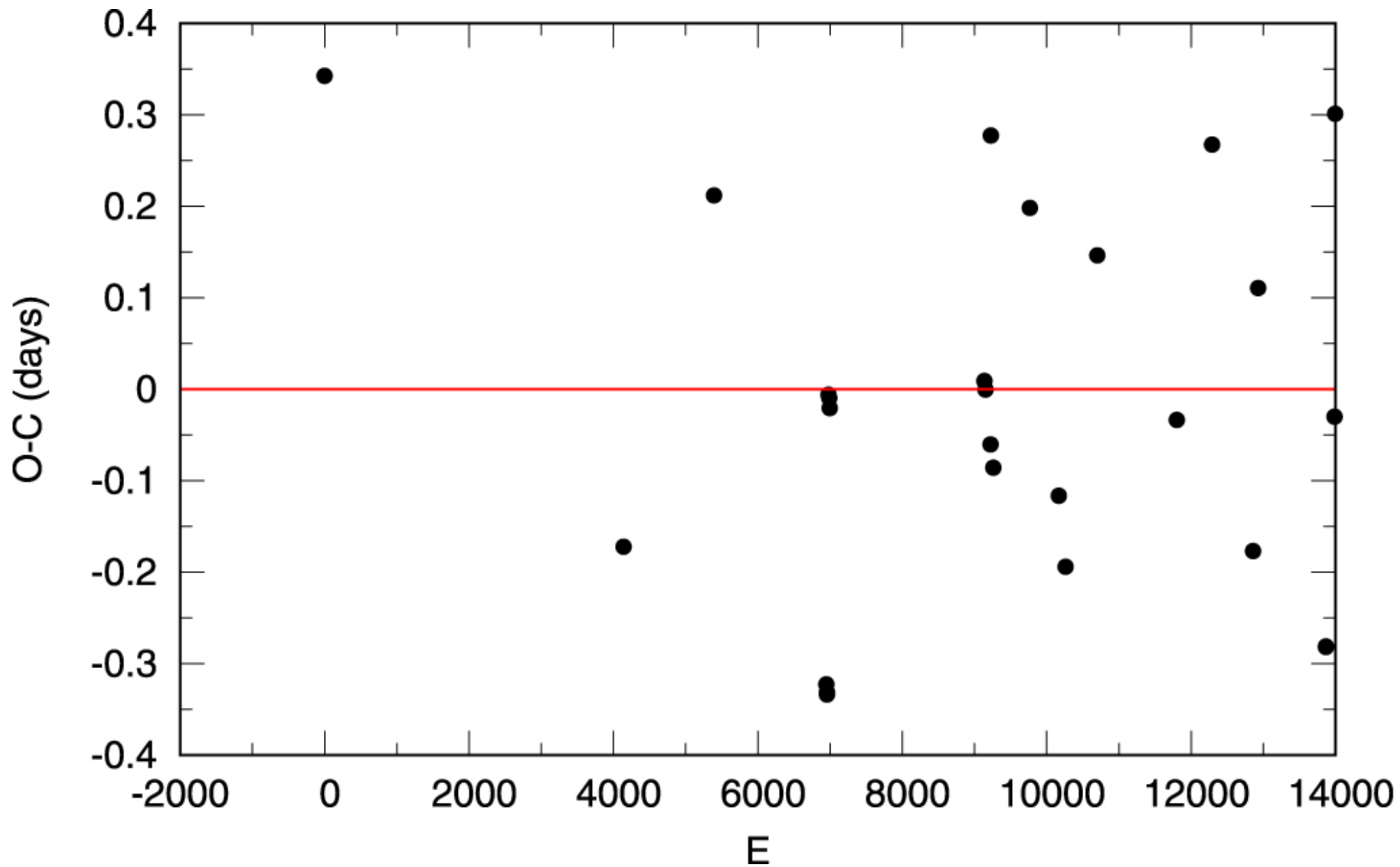
Figure 10. from C. C. Cortés et al 2024 Astron. J. 167 doi:10.3847/1538-3881/ad0b81 https://dx.doi.org/10.3847/1538-3881/ad0b81 © 2023. The Author(s). Published by the American Astronomical Society.
