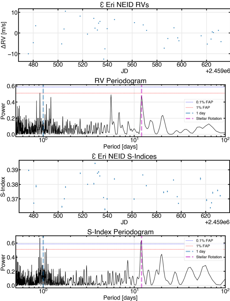
Figure 6. from Sarah Jiang et al 2024 Astron. J. 167 doi:10.3847/1538-3881/ad0b0b https://dx.doi.org/10.3847/1538-3881/ad0b0b © 2023. The Author(s). Published by the American Astronomical Society.
