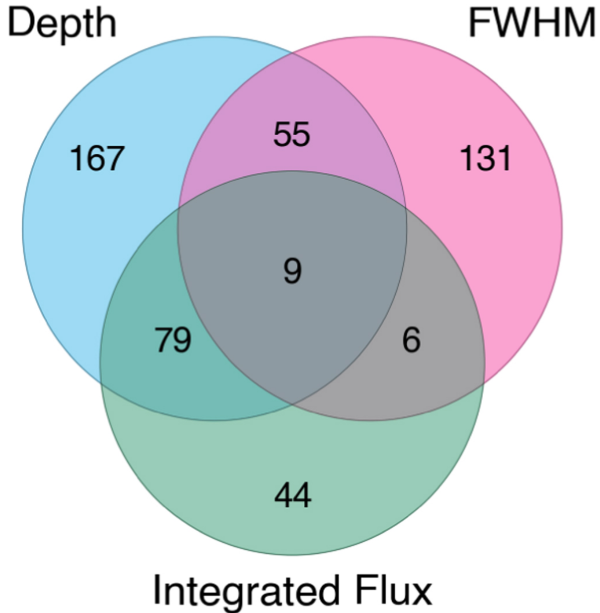
Figure 4. from Sarah Jiang et al 2024 Astron. J. 167 doi:10.3847/1538-3881/ad0b0b https://dx.doi.org/10.3847/1538-3881/ad0b0b © 2023. The Author(s). Published by the American Astronomical Society.
