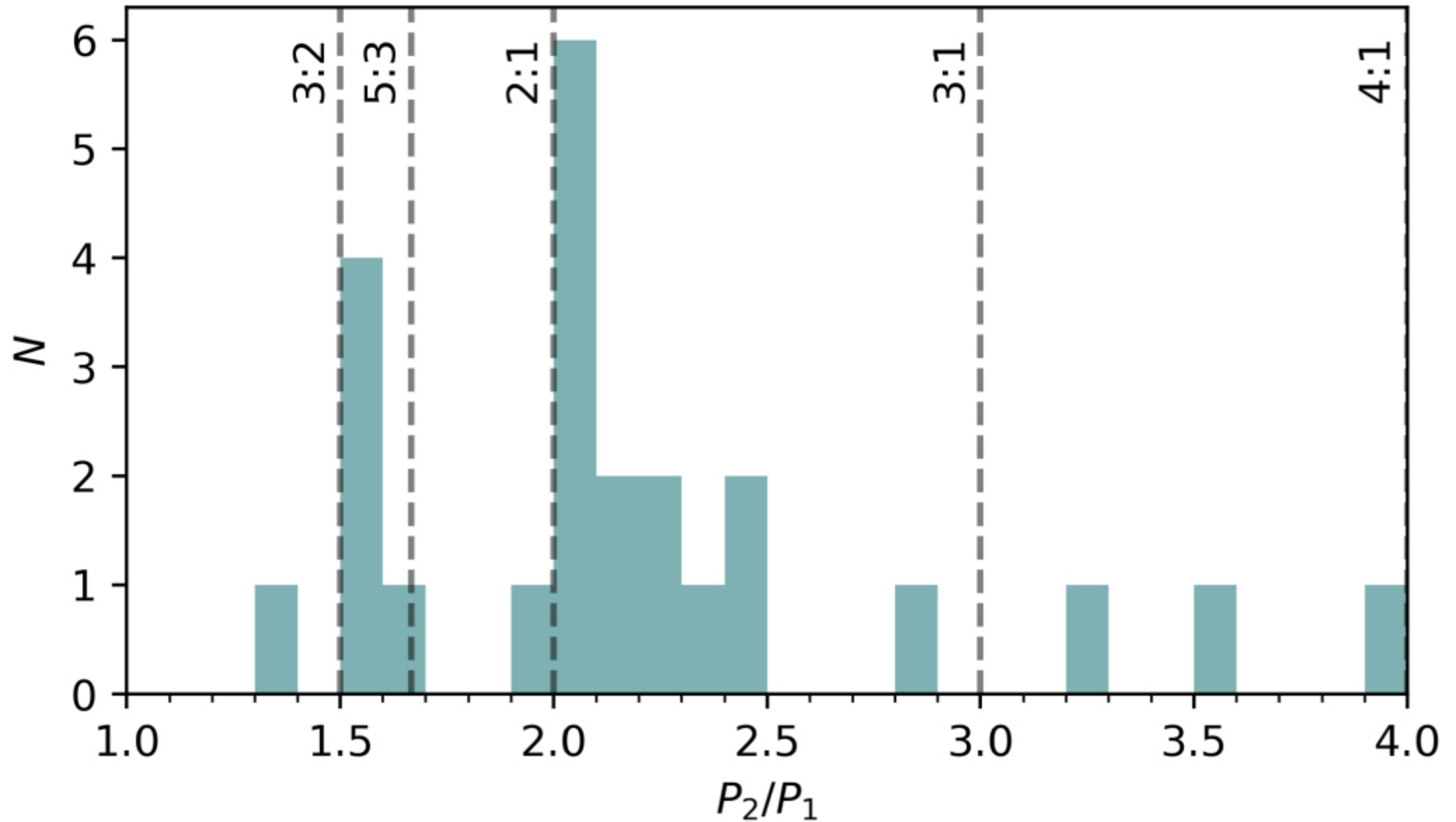
Figure 3. from Malena Rice et al 2023 Astron. J. 166 doi:10.3847/1538-3881/ad09de https://dx.doi.org/10.3847/1538-3881/ad09de © 2023. The Author(s). Published by the American Astronomical Society.
