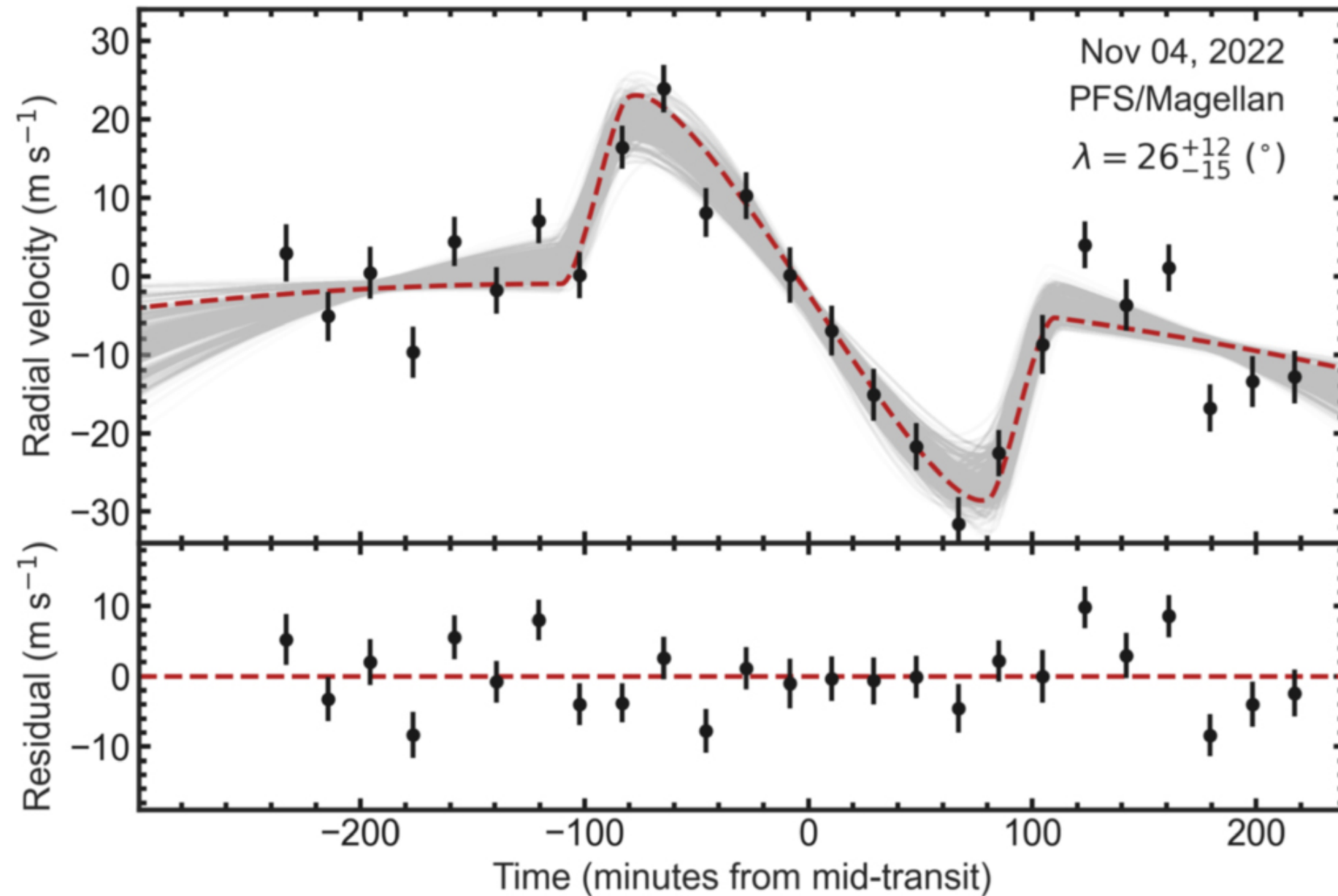
Figure 2. from Malena Rice et al 2023 Astron. J. 166 doi:10.3847/1538-3881/ad09de https://dx.doi.org/10.3847/1538-3881/ad09de © 2023. The Author(s). Published by the American Astronomical Society.
