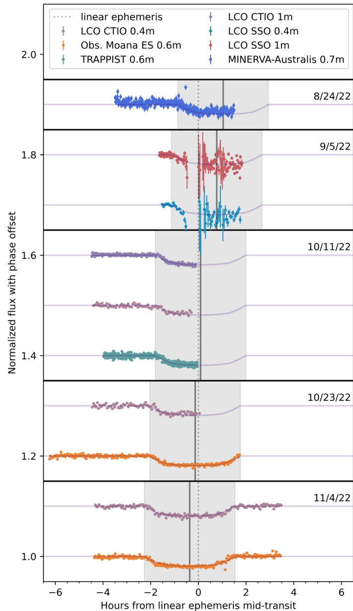
Figure 1. from Malena Rice et al 2023 Astron. J. 166 doi:10.3847/1538-3881/ad09de https://dx.doi.org/10.3847/1538-3881/ad09de © 2023. The Author(s). Published by the American Astronomical Society.
