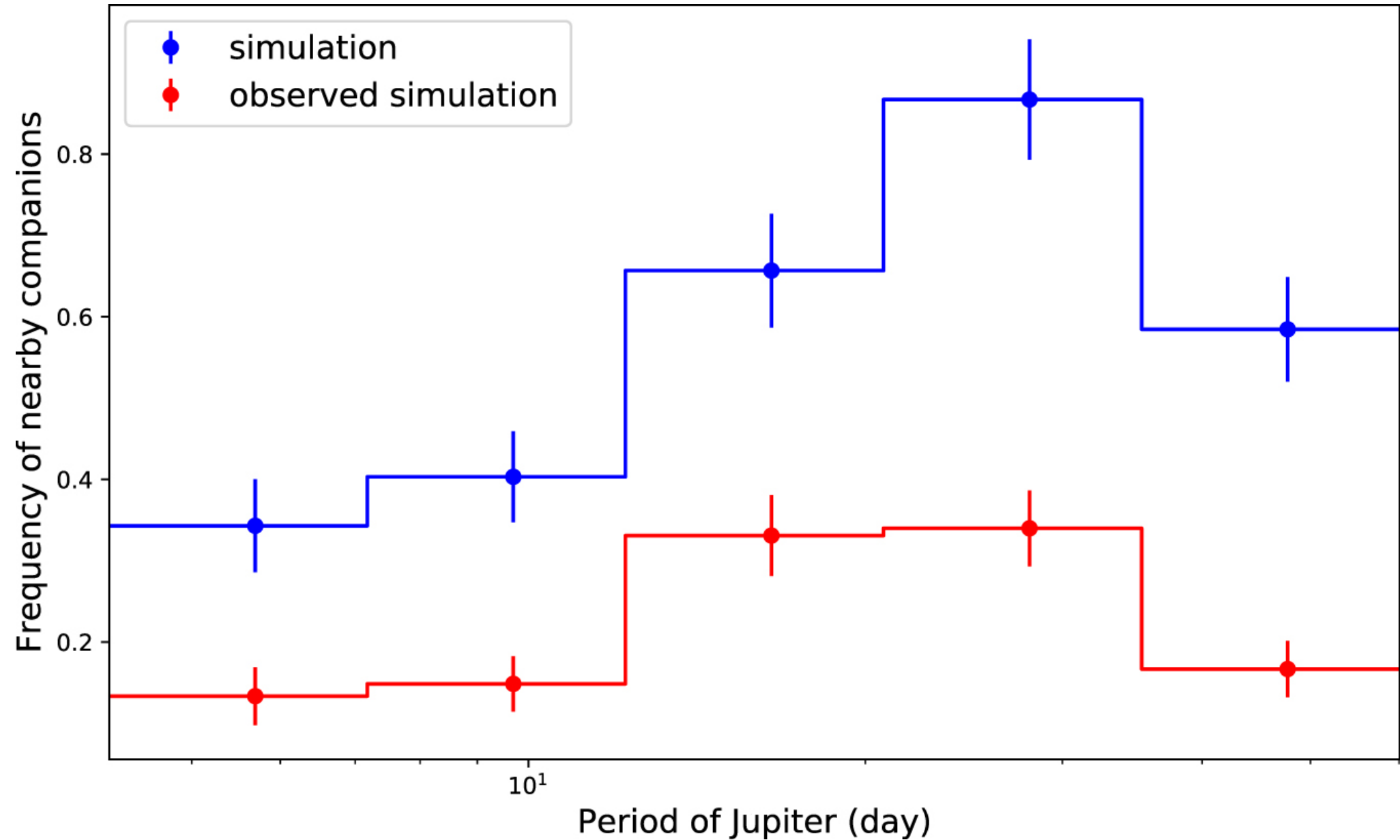
Figure 4. from Dong-Hong Wu and Ying He 2023 Astron. J. 166 doi:10.3847/1538-3881/ad09b0 https://dx.doi.org/10.3847/1538-3881/ad09b0 © 2023. The Author(s). Published by the American Astronomical Society.
