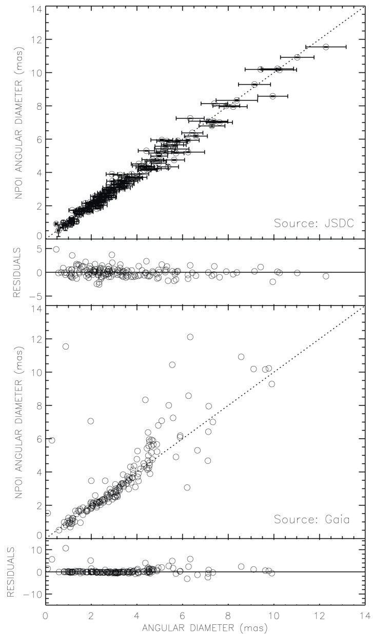
Figure 7. from Ellyn K. Baines et al 2023 Astron. J. 166 doi:10.3847/1538-3881/ad08be https://dx.doi.org/10.3847/1538-3881/ad08be © 2023. The Author(s). Published by the American Astronomical Society.
