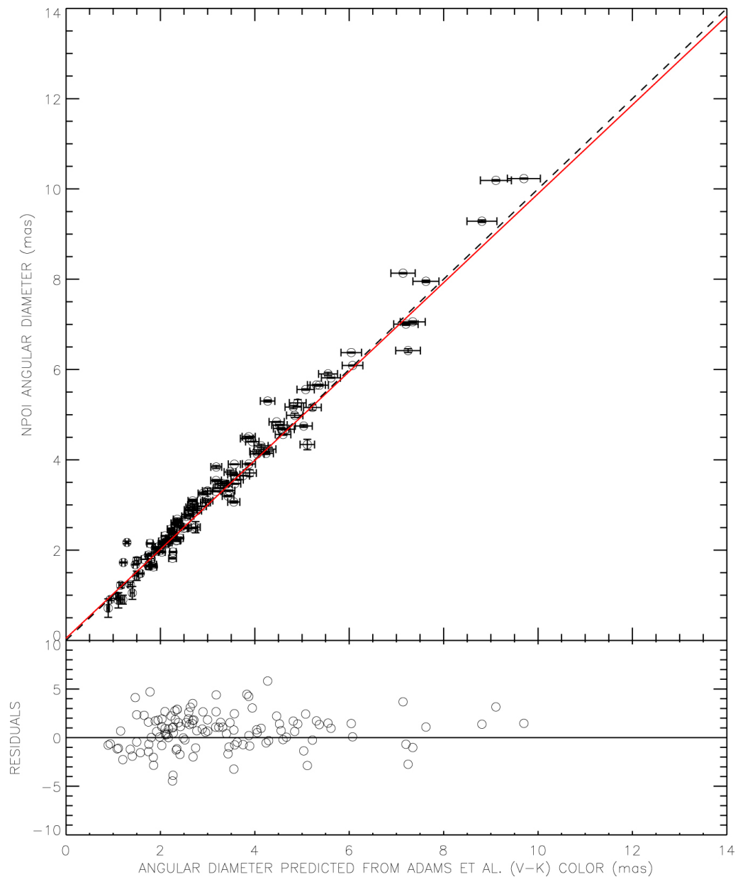
Figure 6. from Ellyn K. Baines et al 2023 Astron. J. 166 doi:10.3847/1538-3881/ad08be https://dx.doi.org/10.3847/1538-3881/ad08be © 2023. The Author(s). Published by the American Astronomical Society.
