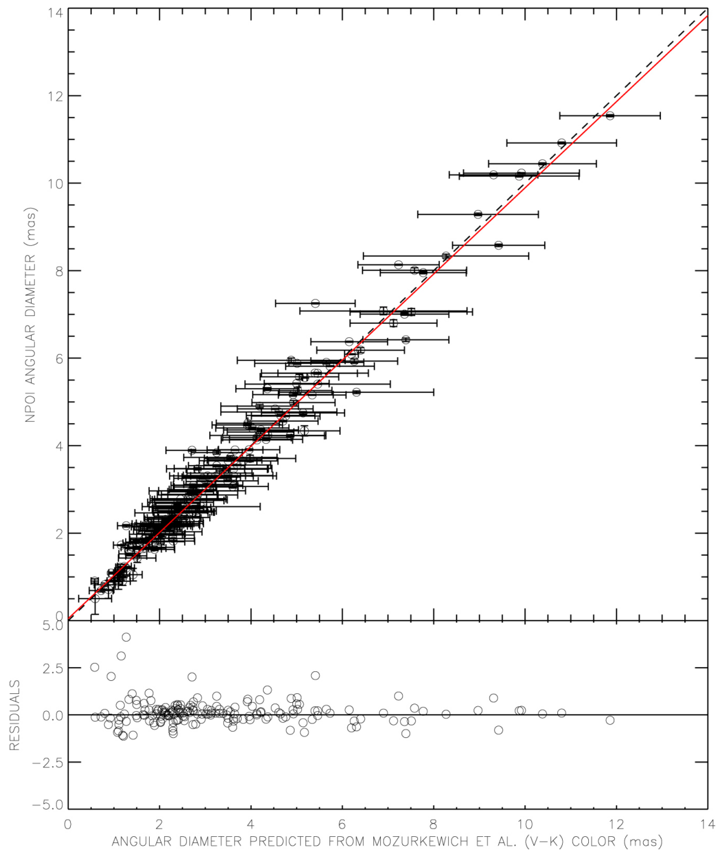
Figure 5. from Ellyn K. Baines et al 2023 Astron. J. 166 doi:10.3847/1538-3881/ad08be https://dx.doi.org/10.3847/1538-3881/ad08be © 2023. The Author(s). Published by the American Astronomical Society.
