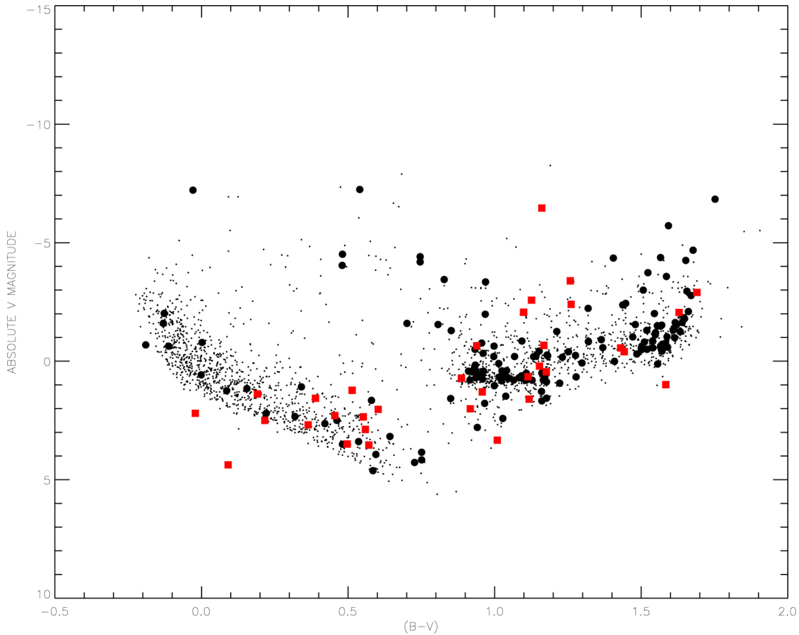
Figure 4. from Ellyn K. Baines et al 2023 Astron. J. 166 doi:10.3847/1538-3881/ad08be https://dx.doi.org/10.3847/1538-3881/ad08be © 2023. The Author(s). Published by the American Astronomical Society.
