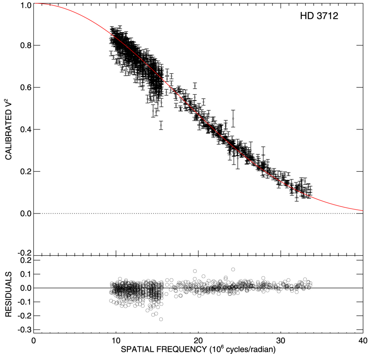
Figure 2. Diameter fits including limb darkening from Ellyn K. Baines et al 2023 Astron. J. 166 doi:10.3847/1538-3881/ad08be https://dx.doi.org/10.3847/1538-3881/ad08be © 2023. The Author(s). Published by the American Astronomical Society.
