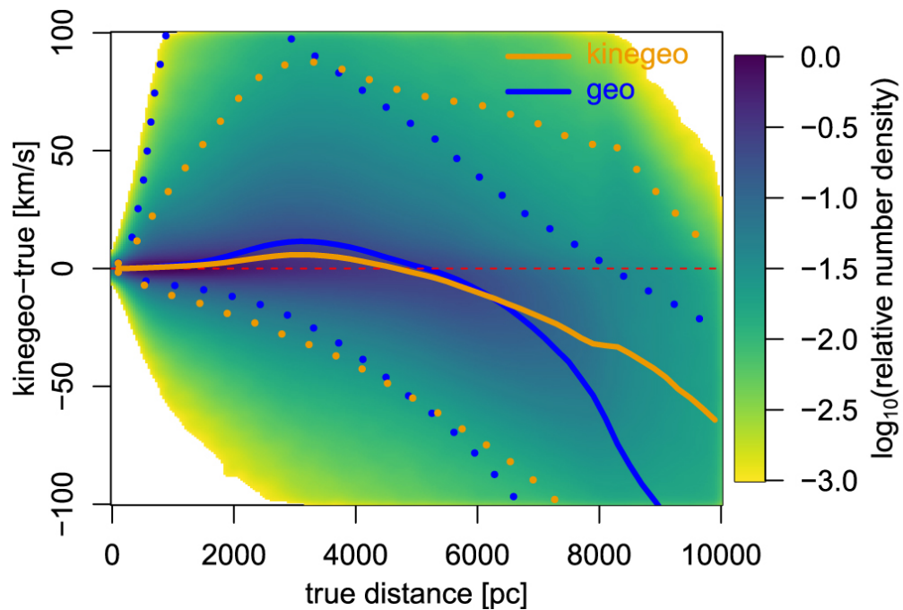
Figure 9. from C. A. L. Bailer-Jones 2023 Astron. J. 166 doi:10.3847/1538-3881/ad08bb https://dx.doi.org/10.3847/1538-3881/ad08bb © 2023. The Author(s). Published by the American Astronomical Society.
