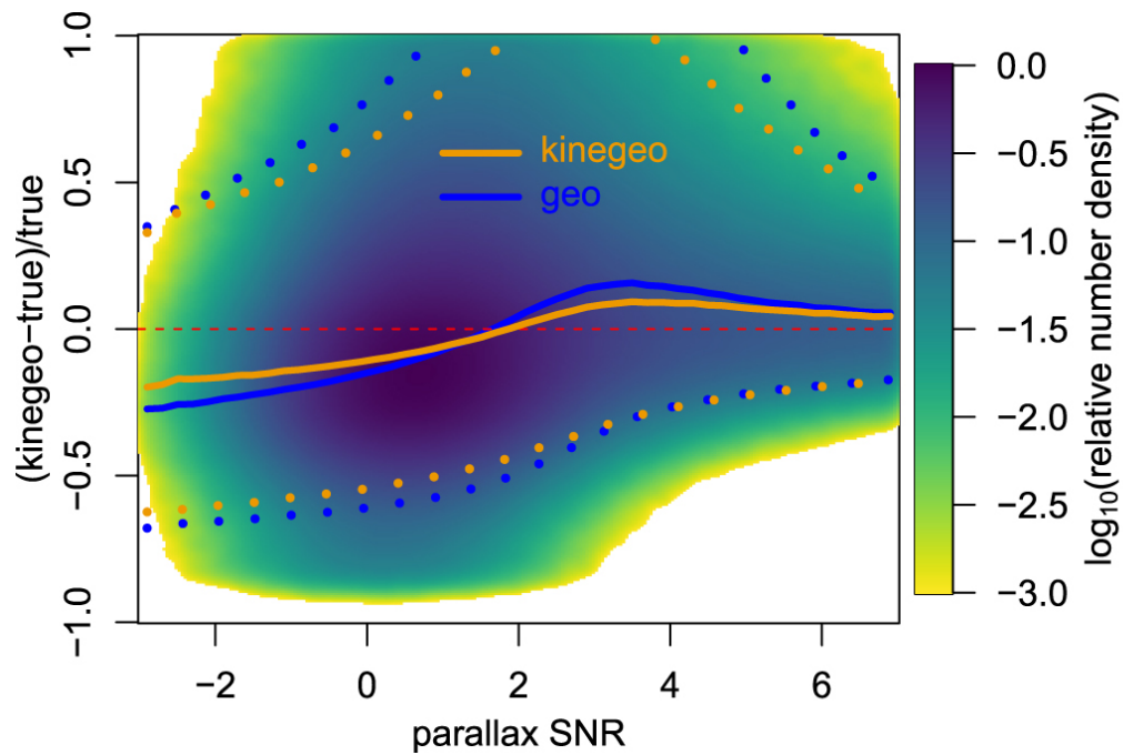
Figure 8. from C. A. L. Bailer-Jones 2023 Astron. J. 166 doi:10.3847/1538-3881/ad08bb https://dx.doi.org/10.3847/1538-3881/ad08bb © 2023. The Author(s). Published by the American Astronomical Society.
