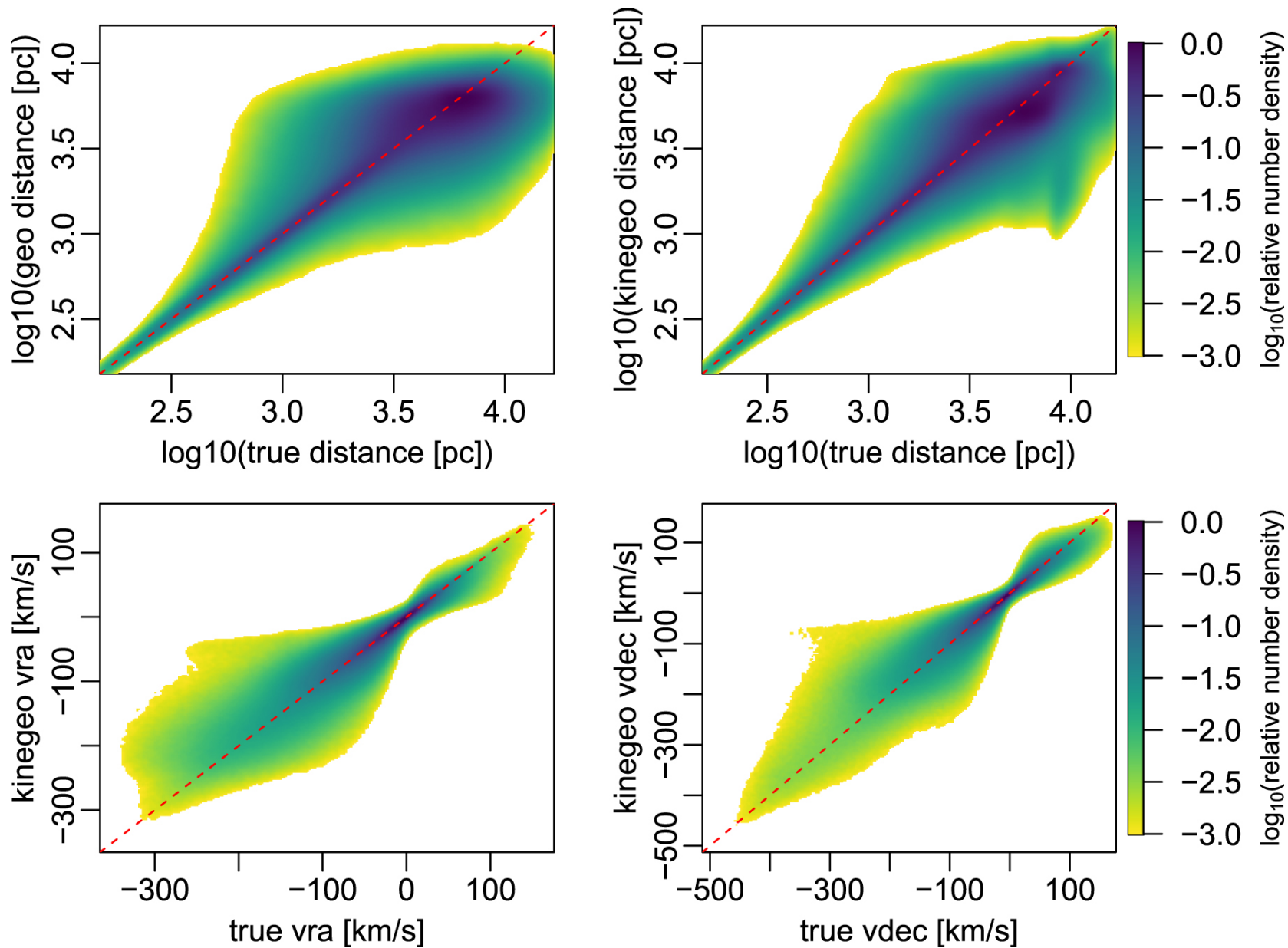
Figure 6. from C. A. L. Bailer-Jones 2023 Astron. J. 166 doi:10.3847/1538-3881/ad08bb https://dx.doi.org/10.3847/1538-3881/ad08bb © 2023. The Author(s). Published by the American Astronomical Society.
