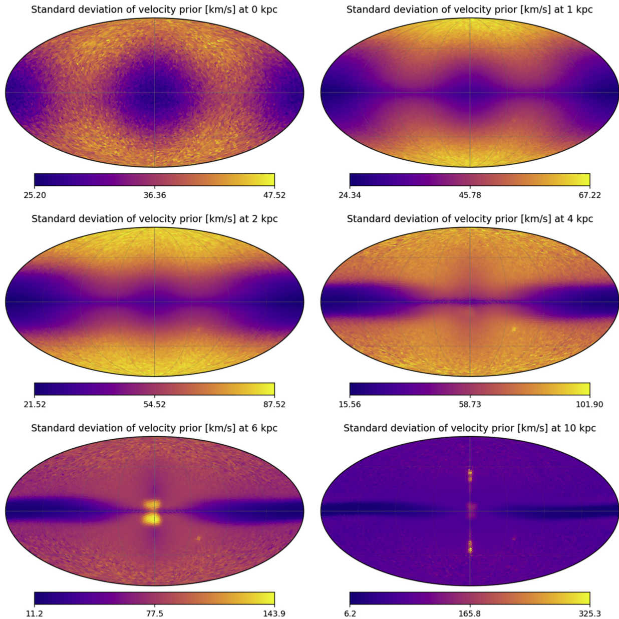
Figure 5. from C. A. L. Bailer-Jones 2023 Astron. J. 166 doi:10.3847/1538-3881/ad08bb https://dx.doi.org/10.3847/1538-3881/ad08bb © 2023. The Author(s). Published by the American Astronomical Society.
