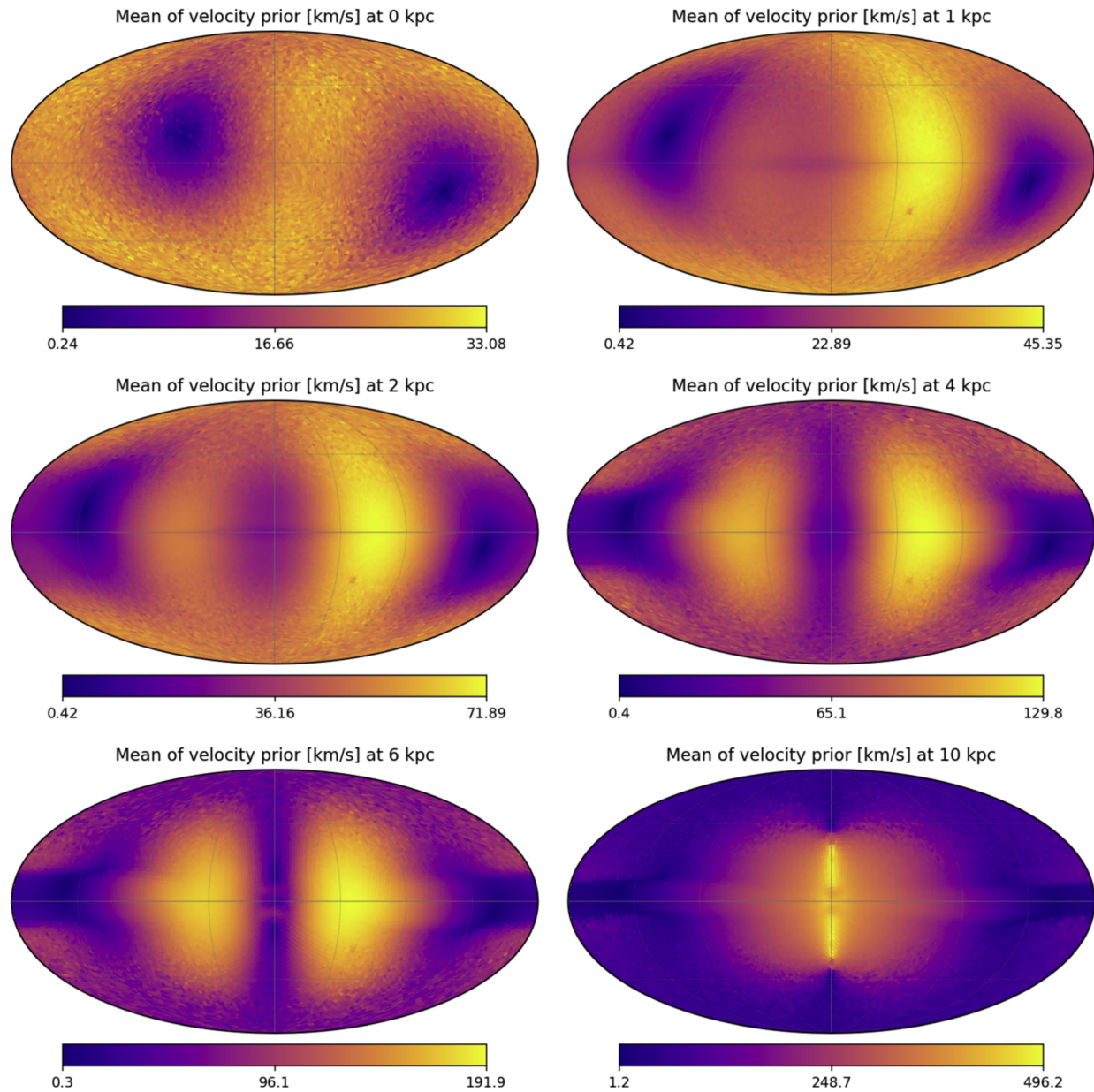
Figure 4. from C. A. L. Bailer-Jones 2023 Astron. J. 166 doi:10.3847/1538-3881/ad08bb https://dx.doi.org/10.3847/1538-3881/ad08bb © 2023. The Author(s). Published by the American Astronomical Society.
