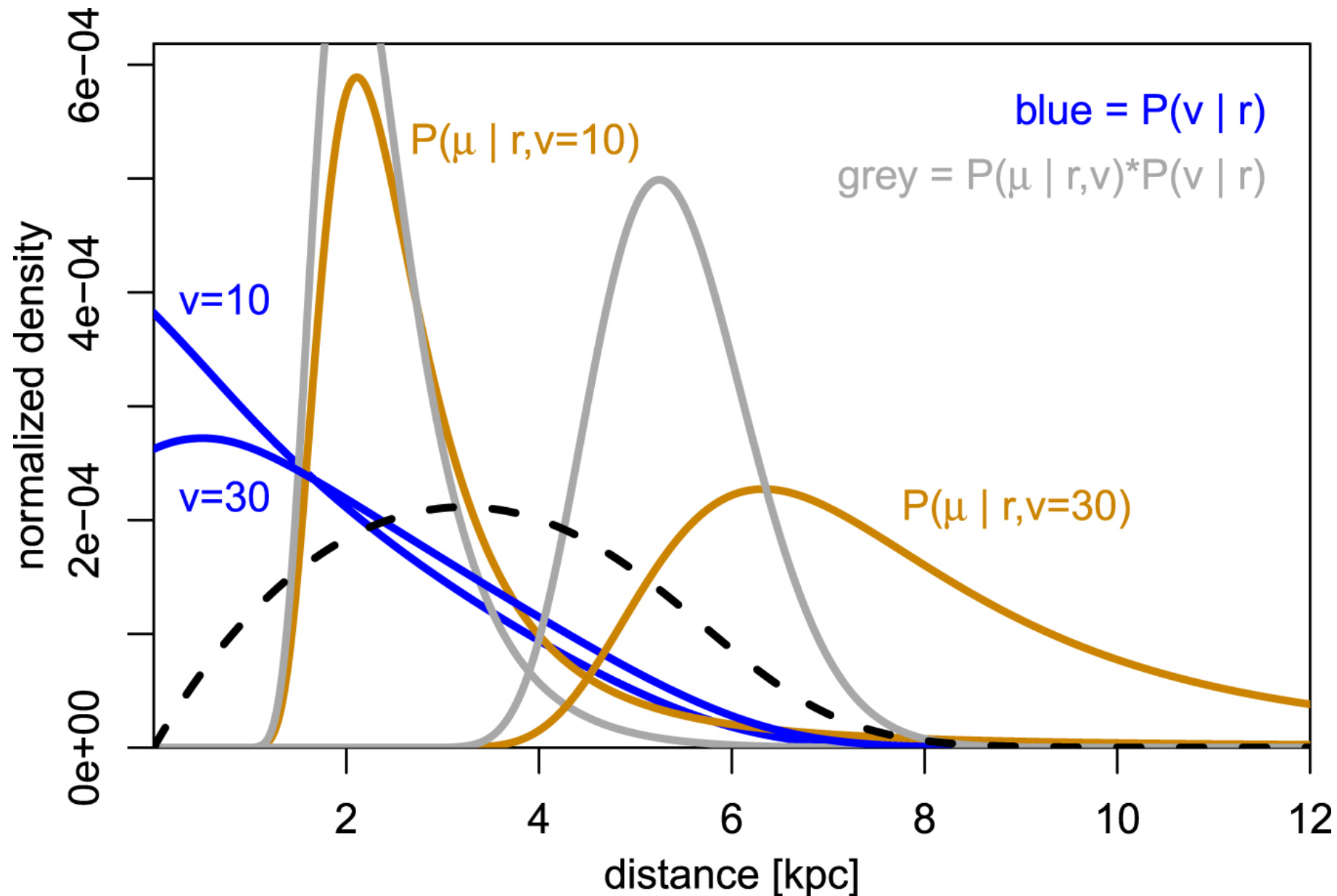
Figure 20. from C. A. L. Bailer-Jones 2023 Astron. J. 166 doi:10.3847/1538-3881/ad08bb https://dx.doi.org/10.3847/1538-3881/ad08bb © 2023. The Author(s). Published by the American Astronomical Society.
