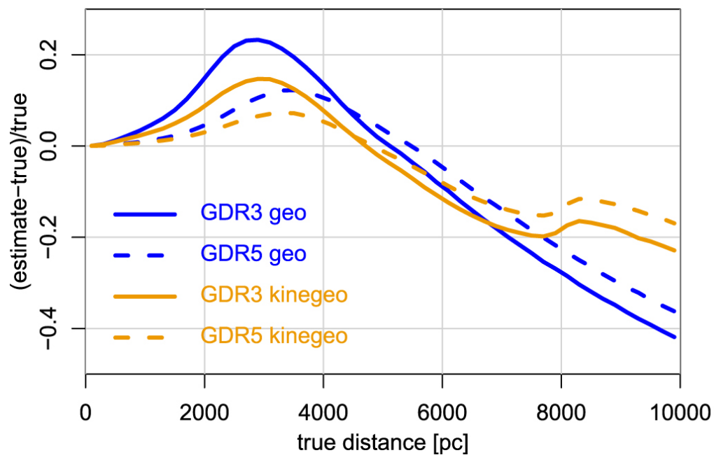
Figure 19. from C. A. L. Bailer-Jones 2023 Astron. J. 166 doi:10.3847/1538-3881/ad08bb https://dx.doi.org/10.3847/1538-3881/ad08bb © 2023. The Author(s). Published by the American Astronomical Society.
