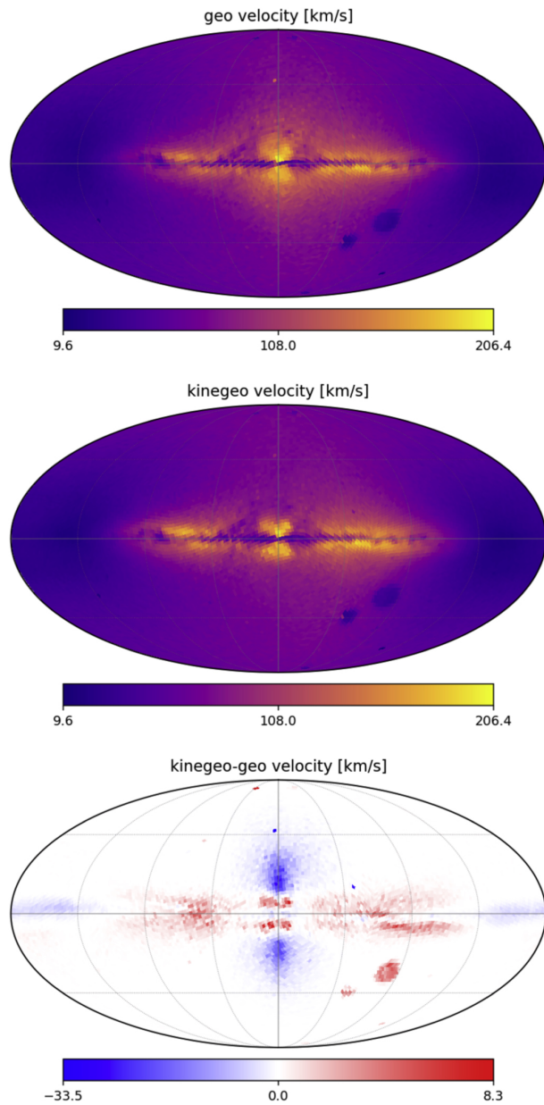
Figure 18. from C. A. L. Bailer-Jones 2023 Astron. J. 166 doi:10.3847/1538-3881/ad08bb https://dx.doi.org/10.3847/1538-3881/ad08bb © 2023. The Author(s). Published by the American Astronomical Society.
