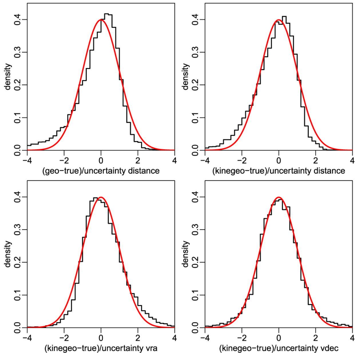
Figure 14. from C. A. L. Bailer-Jones 2023 Astron. J. 166 doi:10.3847/1538-3881/ad08bb https://dx.doi.org/10.3847/1538-3881/ad08bb © 2023. The Author(s). Published by the American Astronomical Society.
