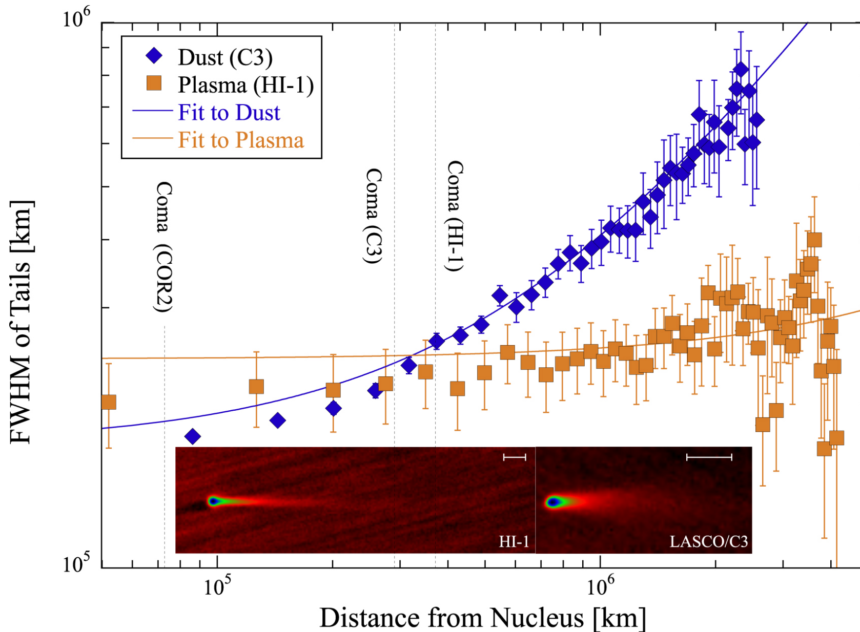
Figure 9. from Jing Li et al 2023 Astron. J. 166 doi:10.3847/1538-3881/ad08af https://dx.doi.org/10.3847/1538-3881/ad08af © 2023. The Author(s). Published by the American Astronomical Society.
