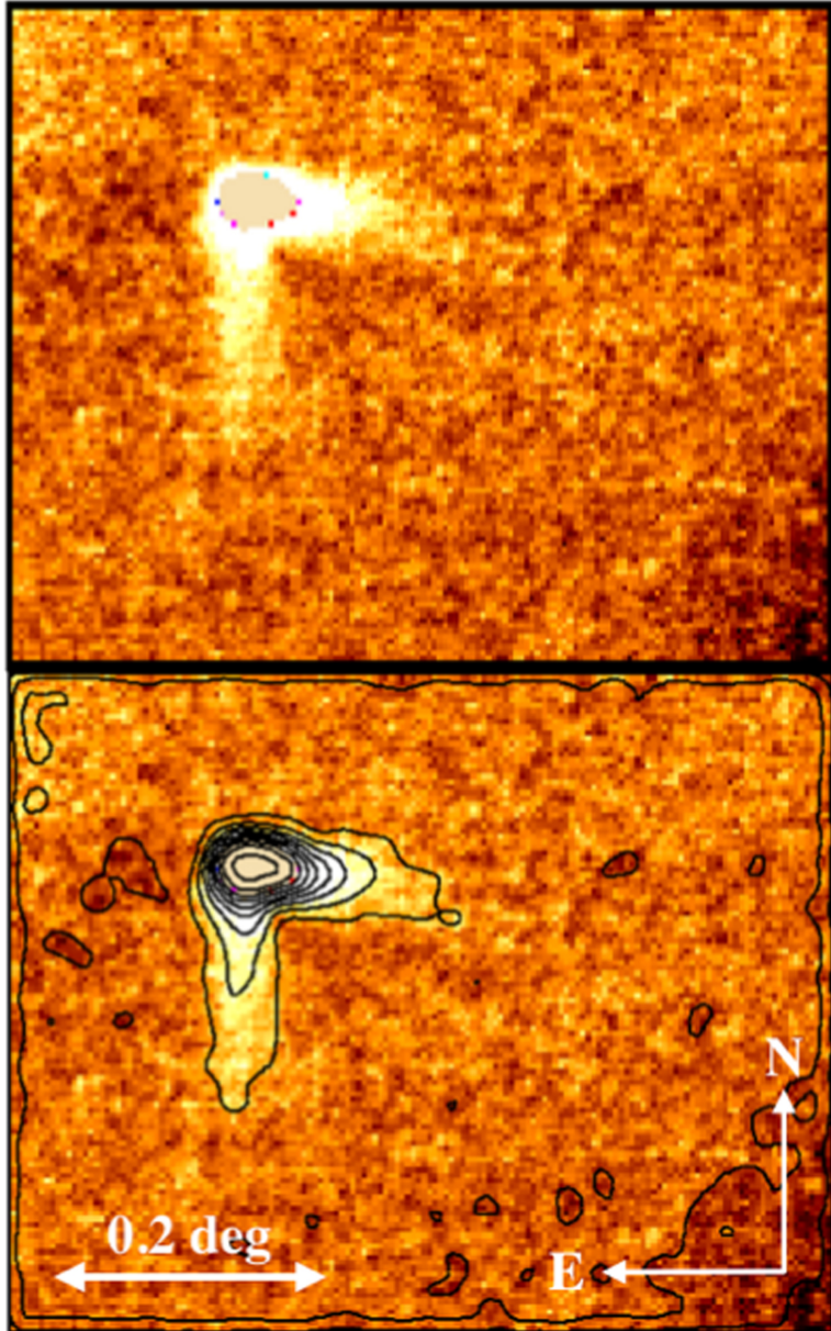
Figure 8. from Jing Li et al 2023 Astron. J. 166 doi:10.3847/1538-3881/ad08af https://dx.doi.org/10.3847/1538-3881/ad08af © 2023. The Author(s). Published by the American Astronomical Society.
