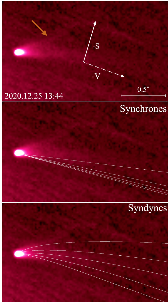
Figure 6. from Jing Li et al 2023 Astron. J. 166 doi:10.3847/1538-3881/ad08af https://dx.doi.org/10.3847/1538-3881/ad08af © 2023. The Author(s). Published by the American Astronomical Society.
