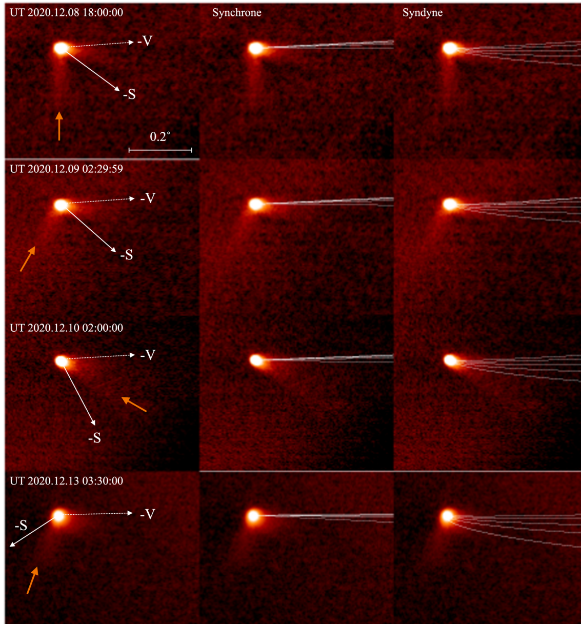
Figure 5. from Jing Li et al 2023 Astron. J. 166 doi:10.3847/1538-3881/ad08af https://dx.doi.org/10.3847/1538-3881/ad08af © 2023. The Author(s). Published by the American Astronomical Society.
